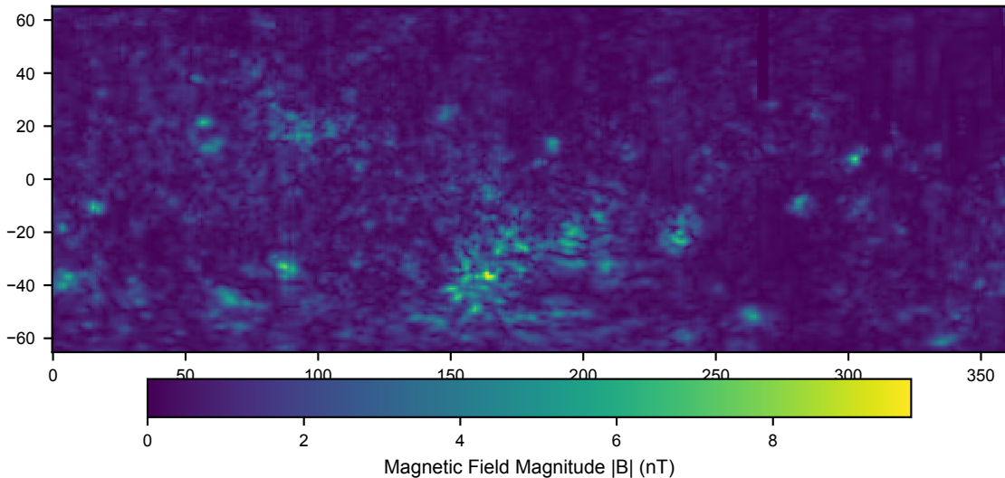
Global Lunar Crustal Magnetic Field
