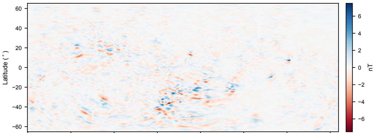
Azimuthal Component ( B_{\phi} )
