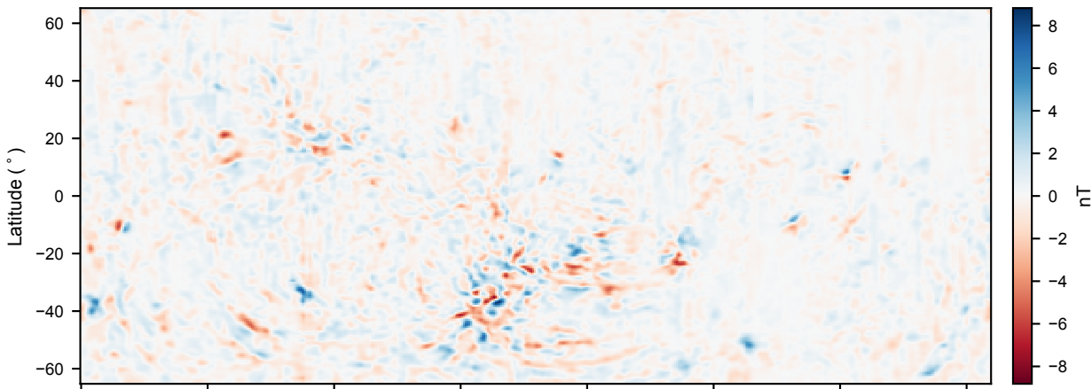
Colatitude Component ( B_{\theta} )
