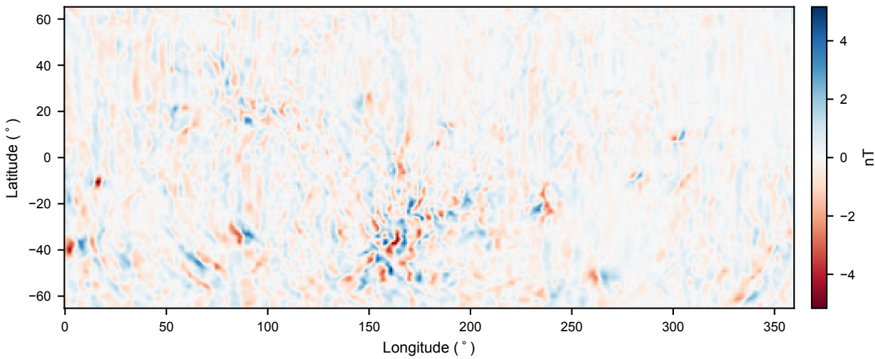
Azimuthal Component ( B_{\phi} )
