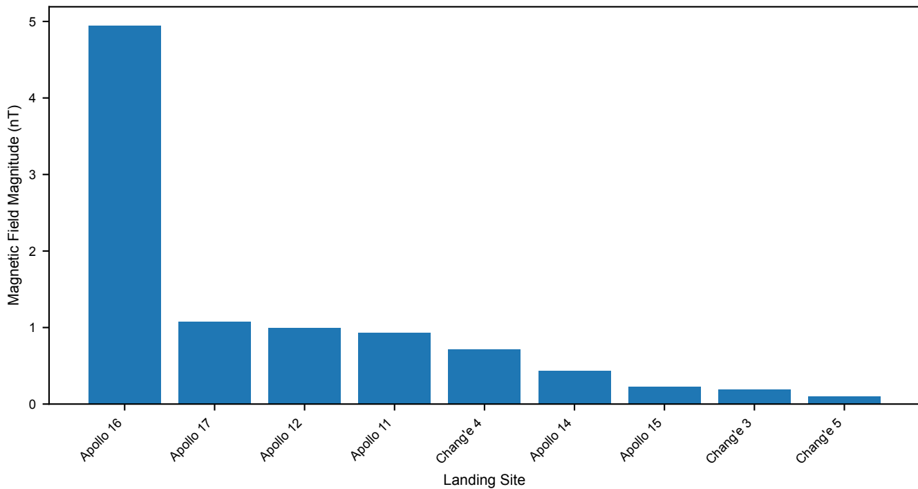
Magnetic Environment at Planned and Historic Landing Sites
