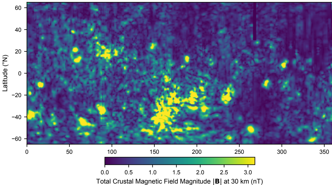
Global Lunar Crustal Magnetic Field Magnitude ( |\mathbf{B}| , 30 km altitude)
