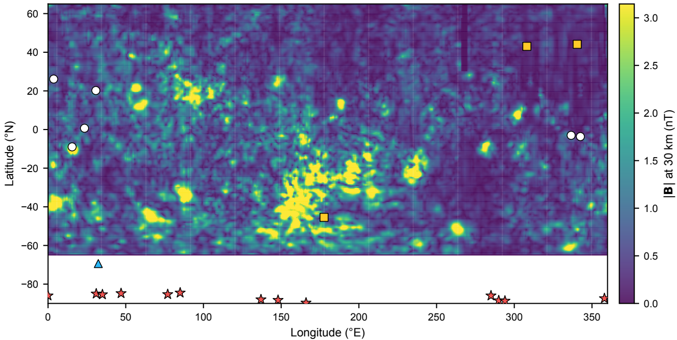
Lunar Landing Sites and Crustal Magnetic Field Distribution
