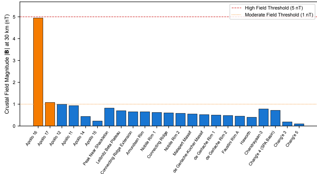
Crustal Magnetic Field Magnitude Across Candidate and Historical Landing Sites
