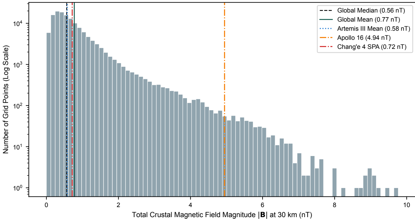
Global Distribution of Lunar Crustal Magnetic Field Magnitude
