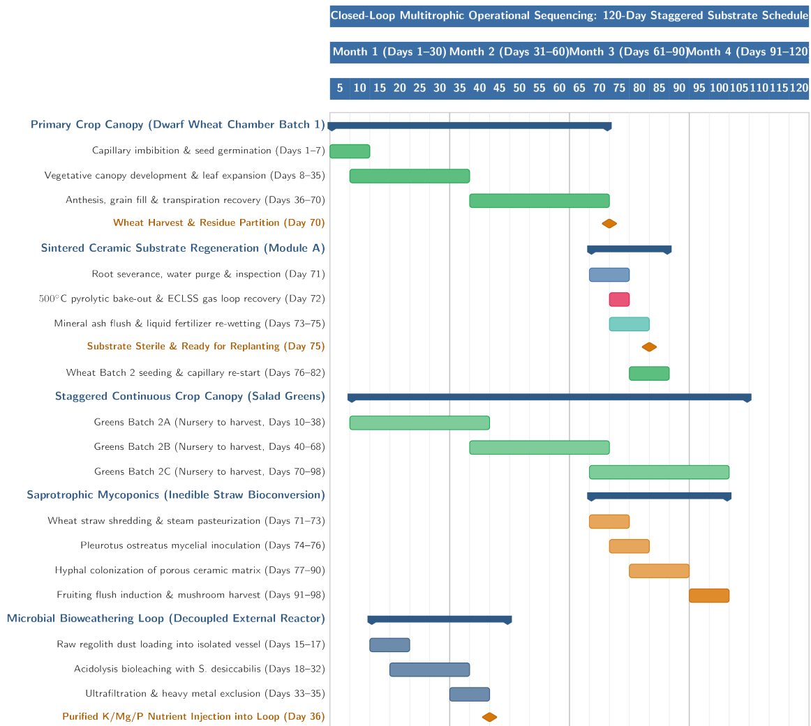
Figure 6. Closed-loop multitrophic operational sequencing and substrate lifecycle schedule. A 120-day repeatable outpost schedule illustrating the temporal coordination between dwarf wheat cultivation (70 days), rapid ceramic substrate pyrolytic regeneration at 500°C with closed-loop CO 2 /moisture recovery (Days 71–75), staggered salad greens production, saprotrophic mushroom ( Pleurotus ostreatus ) bioconversion of inedible straw (Days 71–98), and external microbial bioweathering cycles providing continuous elemental replenishment with zero agricultural downtime.
