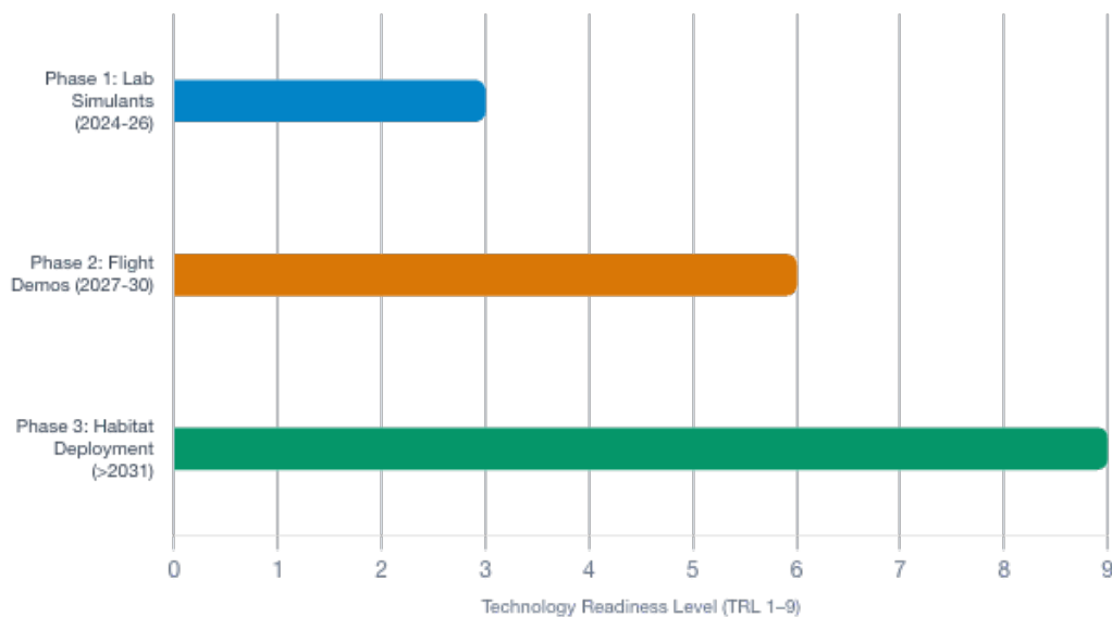
Figure 8. Technology Readiness Level (TRL 1–9) maturation horizon for lunar sintered regolith bio-infrastructure. Strategic progression from Phase 1 laboratory formulations (TRL 1–3, 2024–2026), through Phase 2 subscale flight demonstrations on CLPS landers and the ISS (TRL 4–6, 2027–2030), to Phase 3 operational ISRU habitat integration and closed-loop ECLSS deployment (>2031, TRL 7–9).
