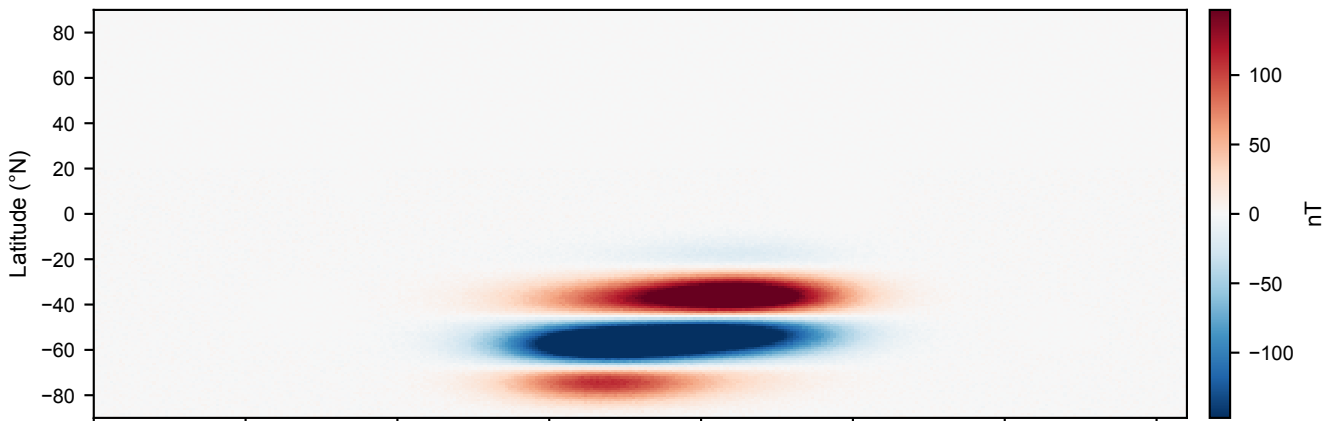
Colatitudinal Component B_{\theta} (Southward)
