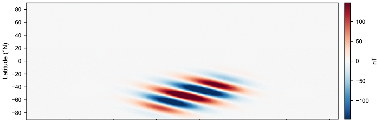
Azimuthal Component B_{\phi} (Eastward)
