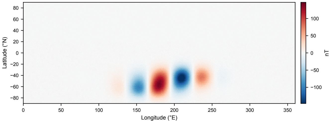
Azimuthal Component B_{\phi} (Eastward)
