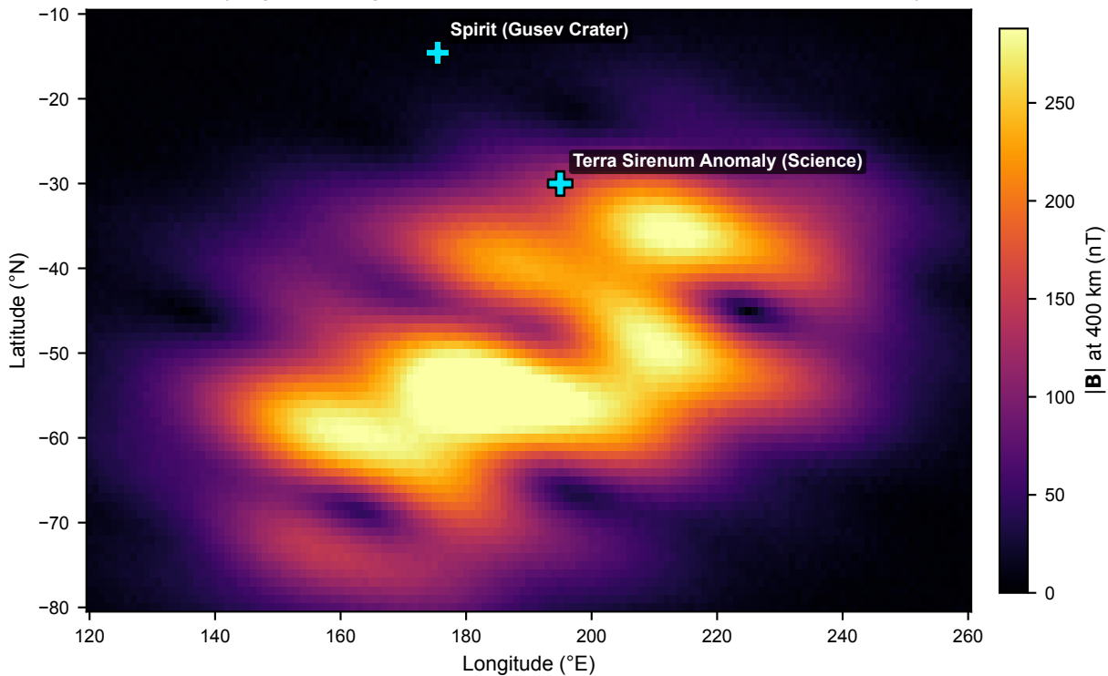
Supplementary Figure S1: High-Resolution Terra Sirenum / Cimmeria Crustal Anomaly Belt
