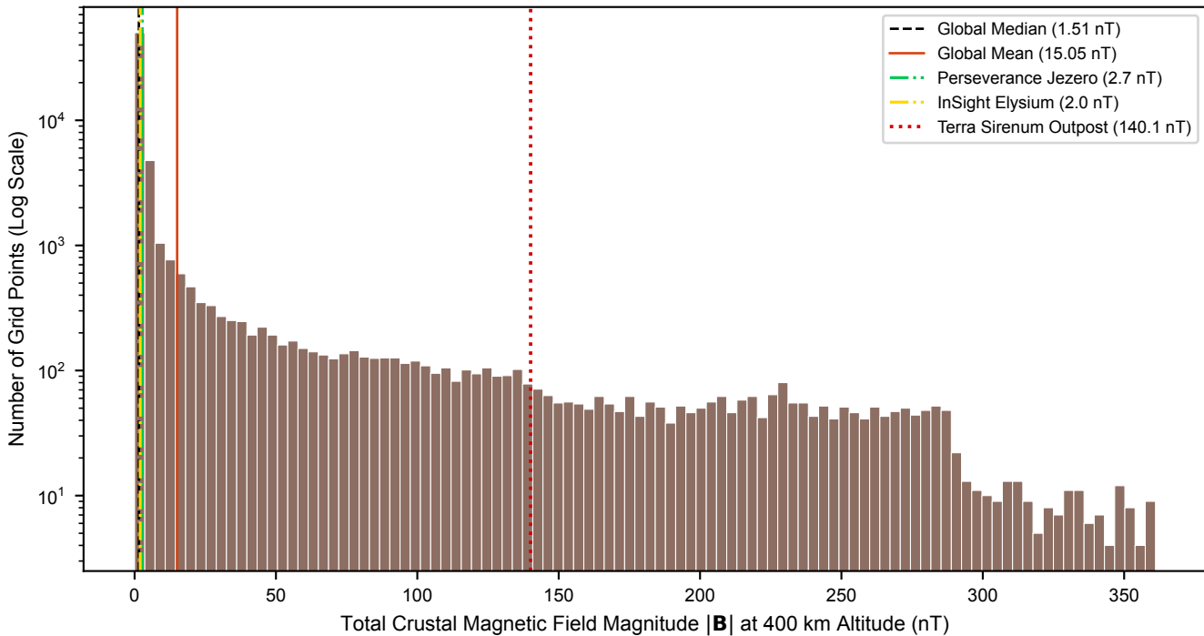
Supplementary Figure S2: Global Distribution of Martian Crustal Magnetic Field Magnitude
