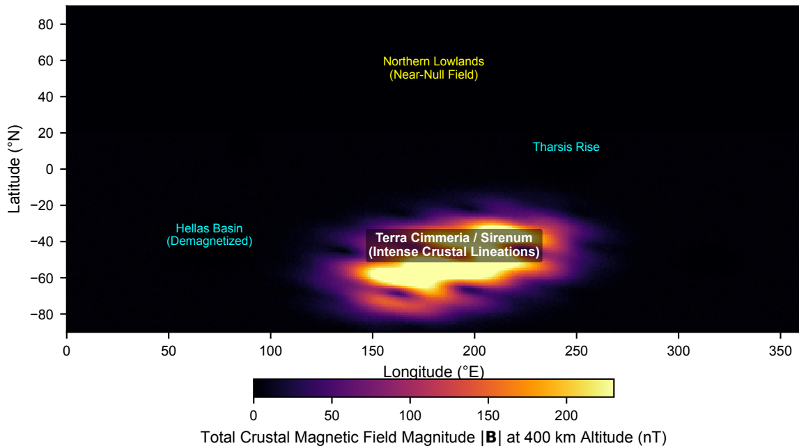
Global Distribution of the Martian Crustal Magnetic Field (Langlais et al. 2019 MAVEN/MGS Model)
