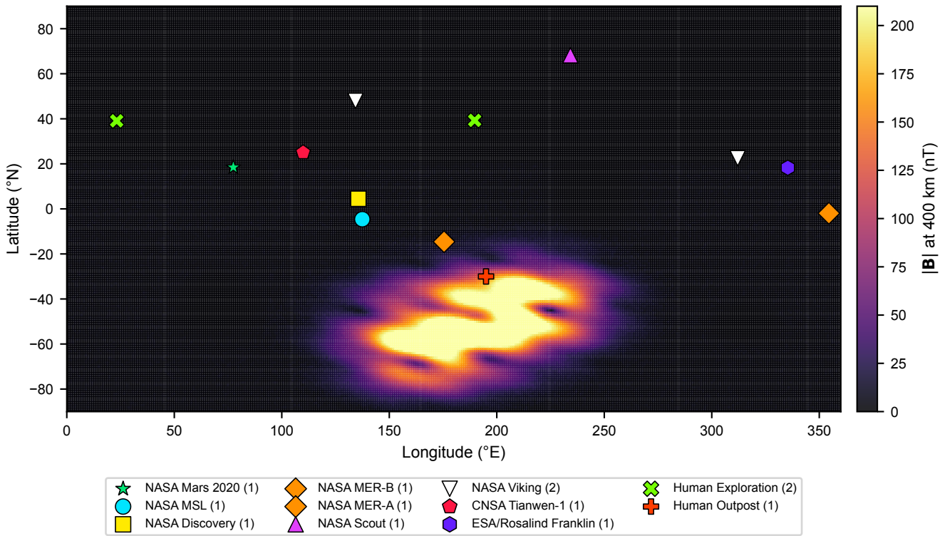
Martian Landing Sites and Candidate Habitats Across Crustal Magnetic Regimes
