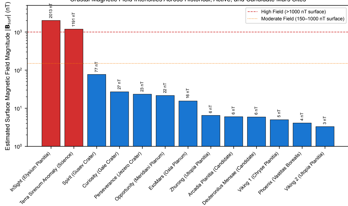
Crustal Magnetic Field Intensities Across Historical, Active, and Candidate Mars Sites
