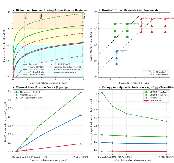
Figure 2 | Richardson number ( Ri ) scaling across gravity fields. a, Ri = Gr/Re^2 trajectories from 1 g to 0 g. b, Gr vs Re regime map. c, Stratification index decay. d, Aerodynamic resistance r_a = 1/g_{bl} .
