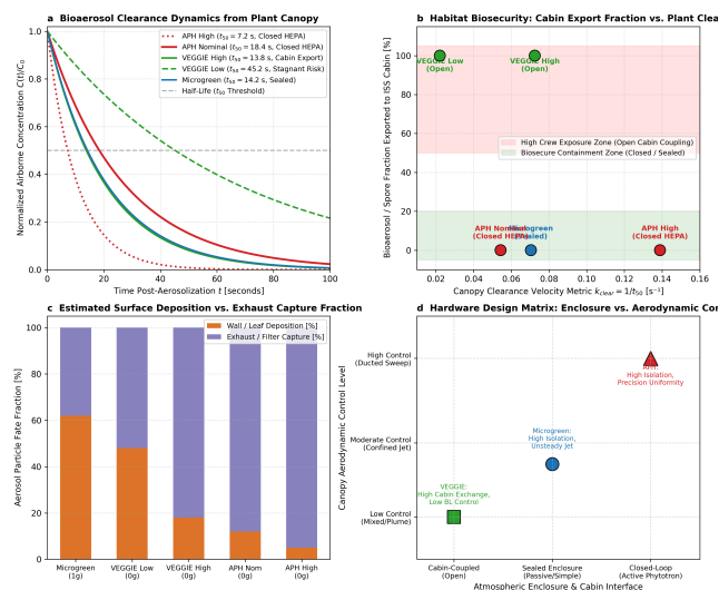
Figure 5 | Habitat biosecurity, bioaerosol clearance, and crew exposure trade space. a , Bioaerosol clearance curves ( C(t)/C_0 ). b , Cabin export percentage vs. clearance rate. c , Surface deposition vs. exhaust filtration. d , Architectural hardware trade matrix.
