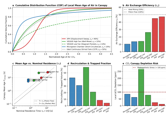
Figure 4 | Scalar ventilation dynamics, Local Mean Age of Air (LMA), and canopy dead zone mapping. a , Cumulative air age CDFs ( \tau_a ). b , Air exchange efficiency ( \epsilon_a ). c , Mean canopy residence time. d , Trapped recirculation fraction. e , Predicted canopy \text{CO}_2 depletion.
