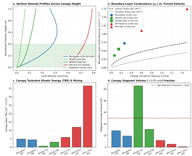
Figure 3 | Canopy boundary-layer conductance and turbulence. a, Vertical velocity profiles u(z) . b, g_{bl} vs forced velocity. c, Canopy TKE. d, Canopy stagnant volume fraction ( U < 0.05 m/s).
