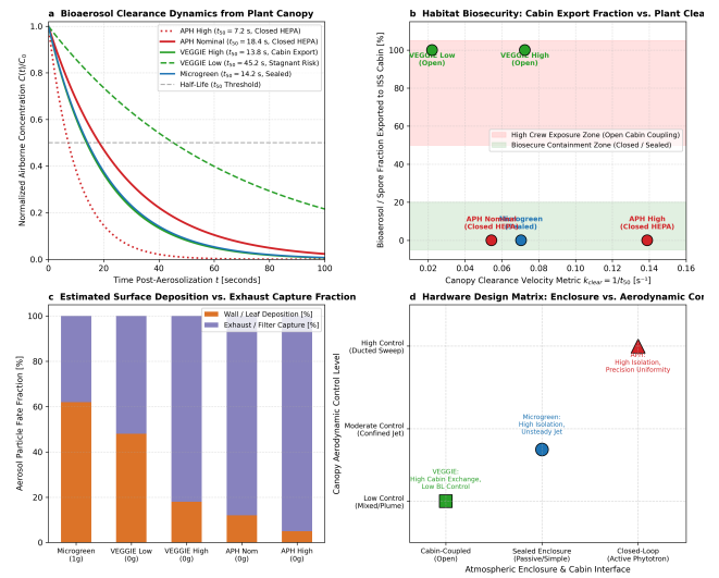
Figure 5 | Habitat biosecurity, bioaerosol clearance, and crew exposure trade space. a, Bioaerosol clearance curves \frac{C(t)}{C_0} . b, Cabin export percentage vs clearance rate. c, Surface deposition vs exhaust filtration. d, Architectural hardware trade matrix.
