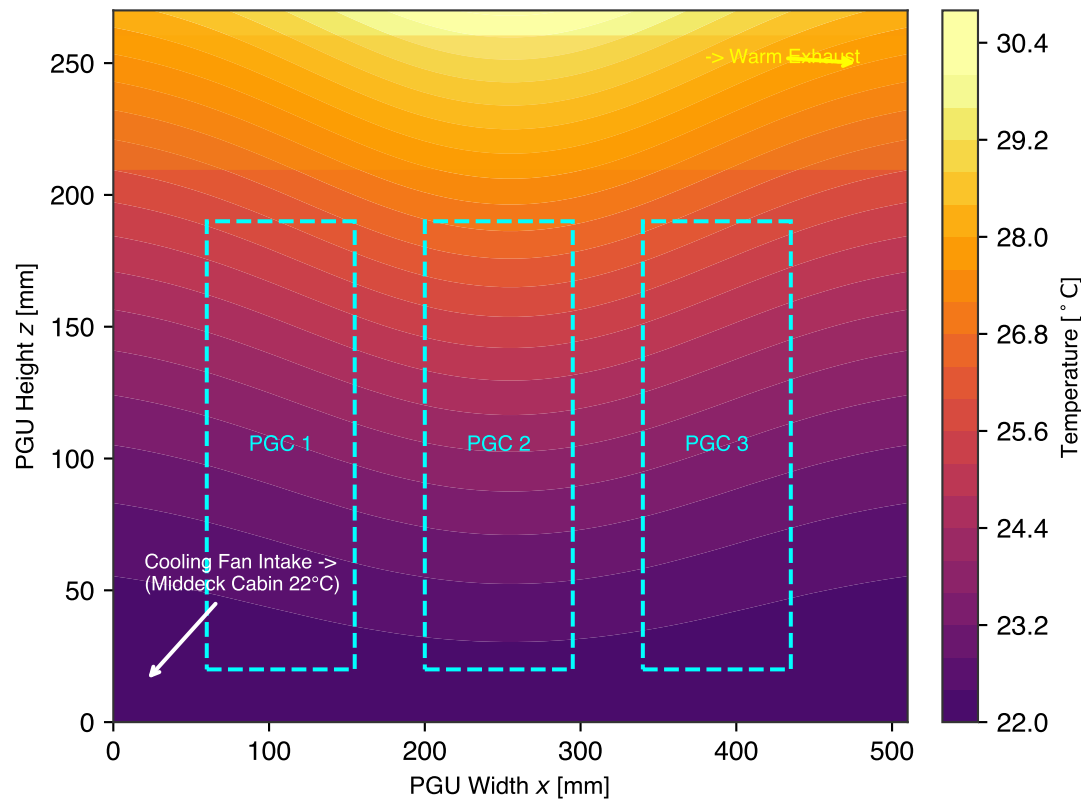
a Macro PGU Middeck Locker Thermal Field ( T [°C])
