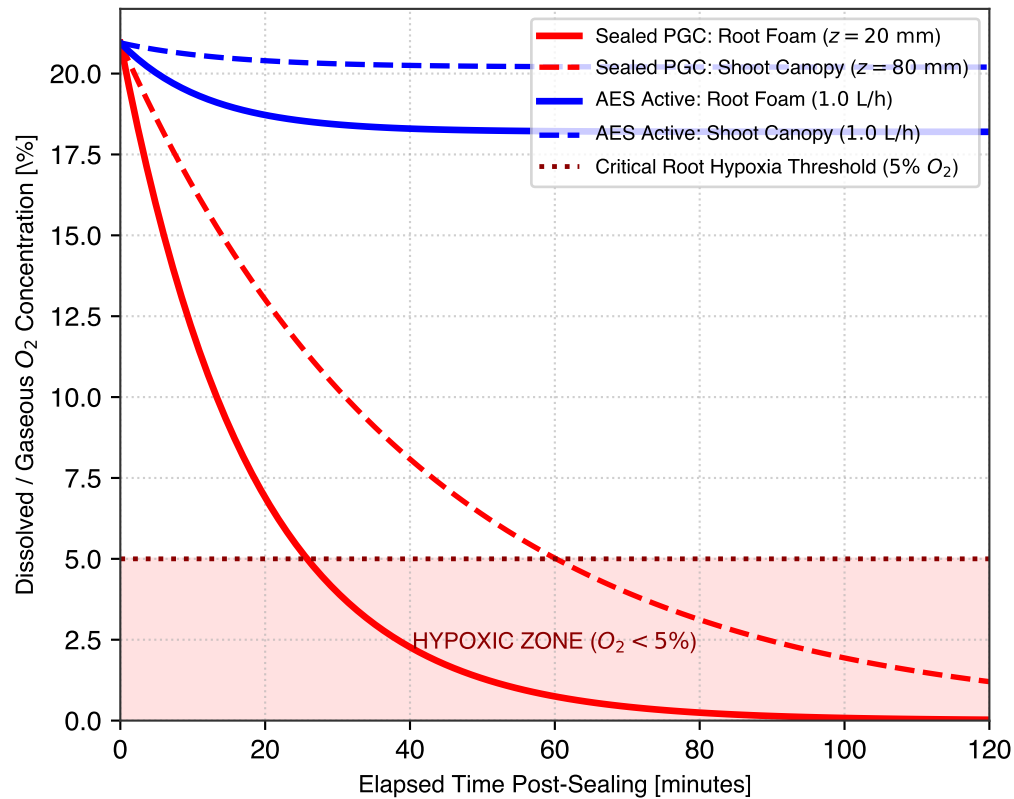
c Transient O_2 Depletion Dynamics (Sealed vs. AES Active)
