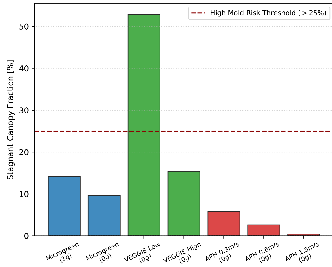
d Canopy Stagnant Volume ( < 0.05 \text{ m/s} ) Fraction
