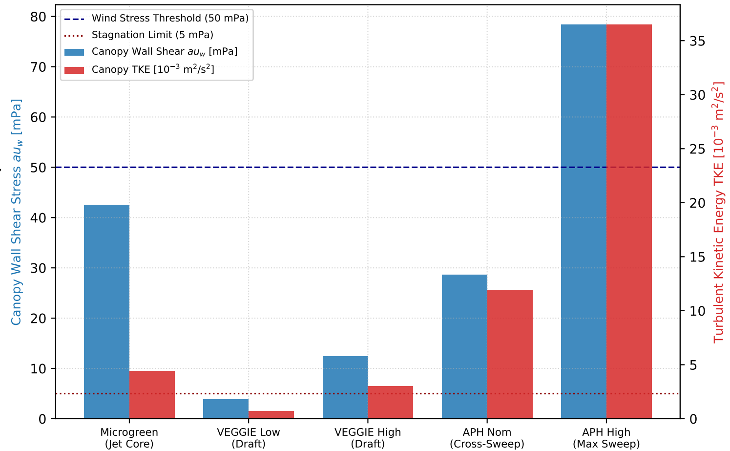
d Canopy Shear Stress ( au_w ) & TKE Penetration
