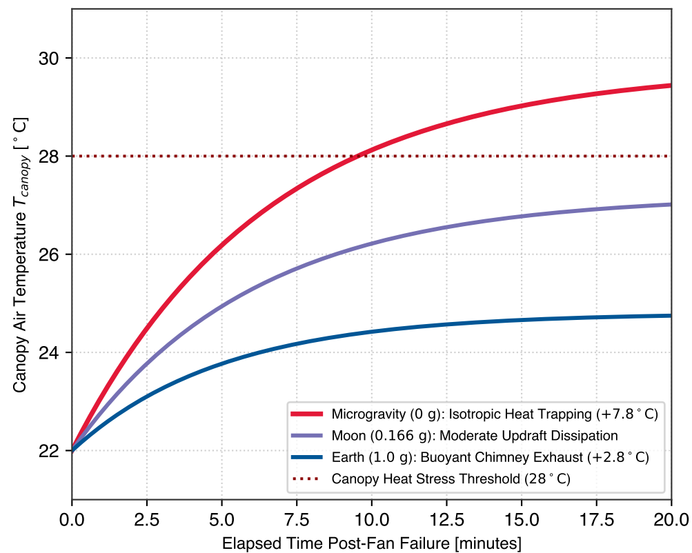
c Canopy Thermal Accumulation Post-Shutdown
