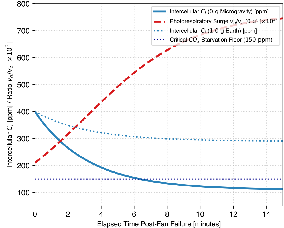
d CO 2 Starvation & RuBisCO Photorespiration Trajectory
