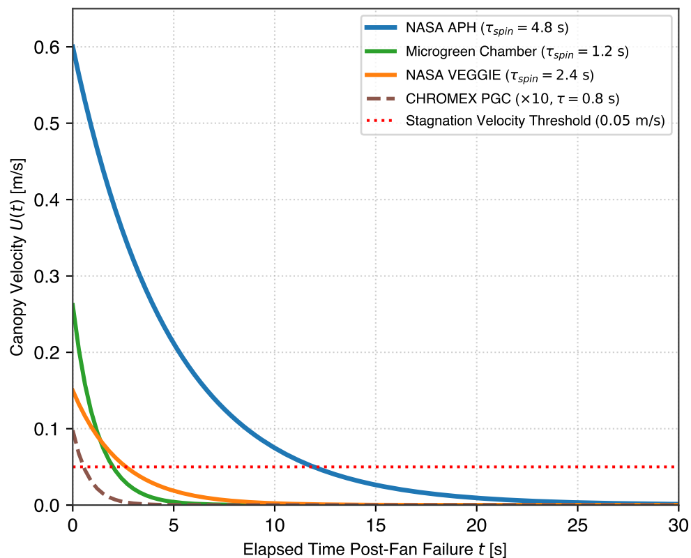
a Fan Spin-Down Velocity Decay Post-Cutoff
