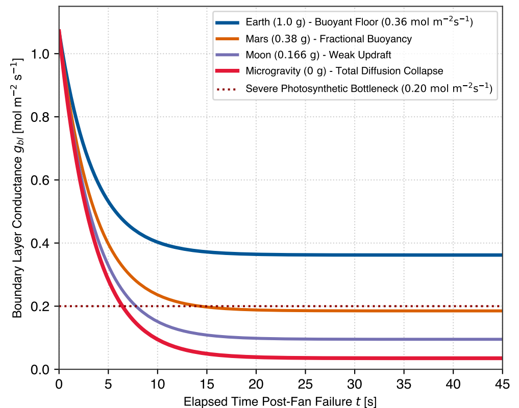
b Aerodynamic Conductance ( g_{bl} ) Collapse Across Gravities
