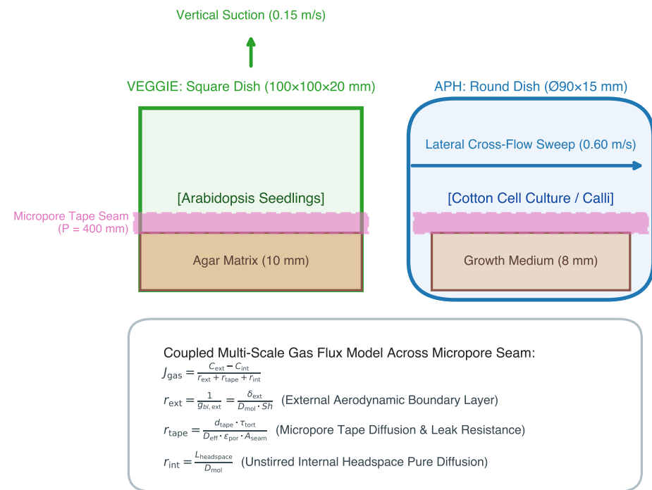
a Sample Carrier Schematics &amp; Micropore Tape Gas Exchange Interfaces
