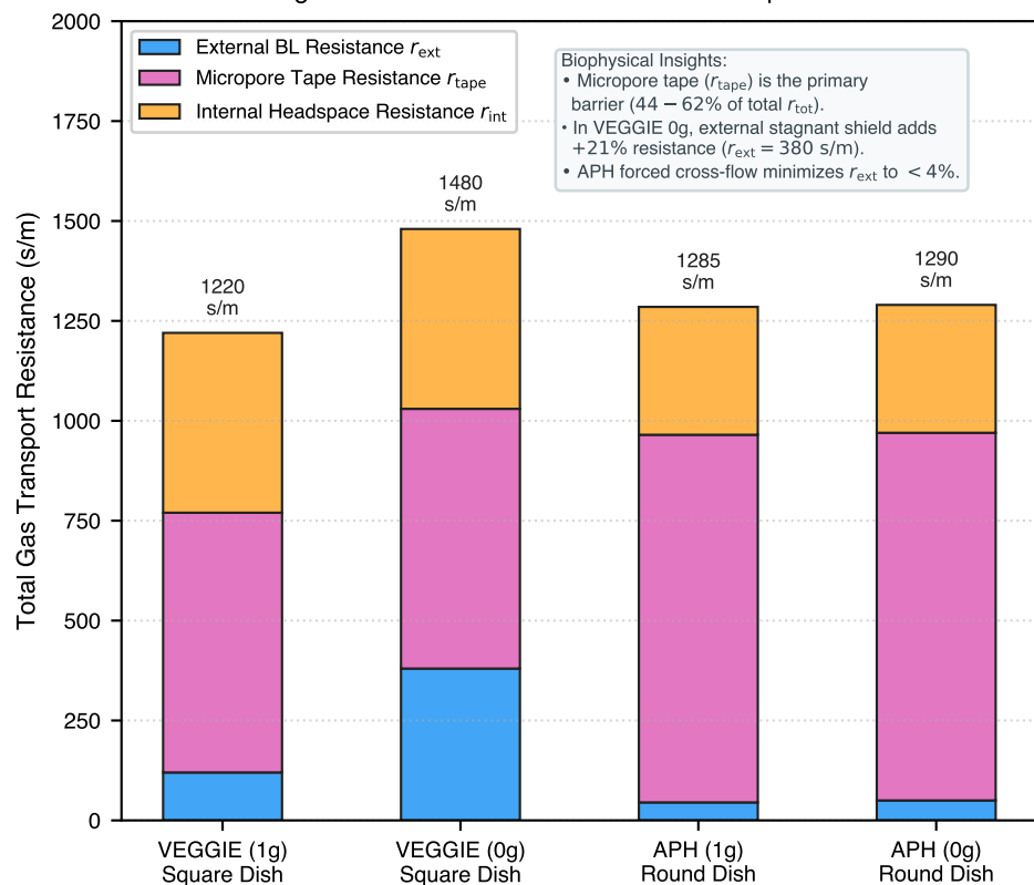
c Gas Exchange Resistance Breakdown Across Transport Barriers
