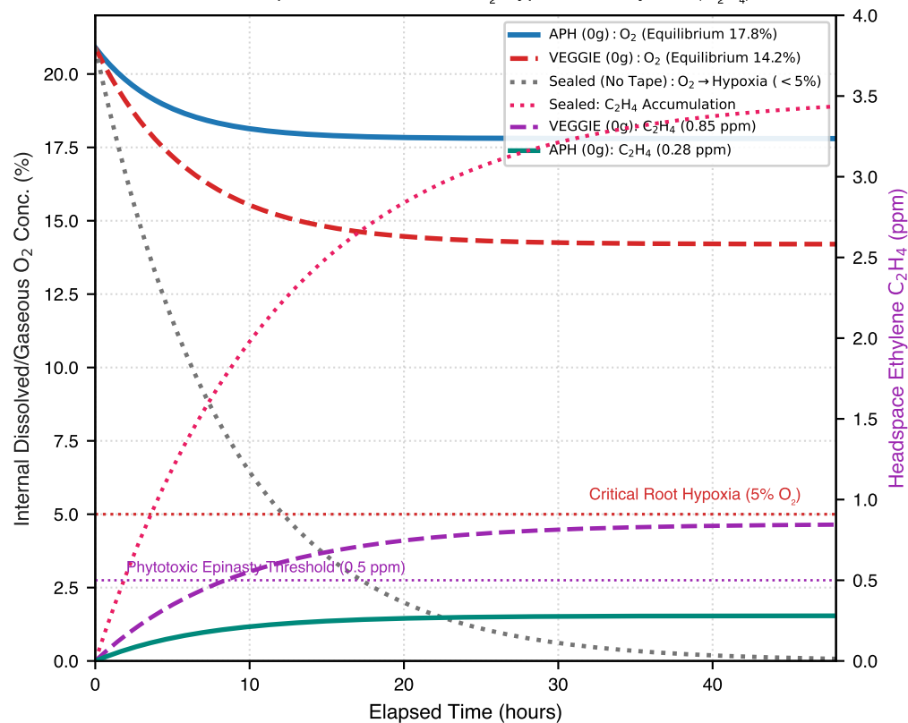
d Transient Headspace Microclimates: \text{O}_2 Hypoxia & Ethylene ( \text{C}_2\text{H}_4 ) Accumulation
