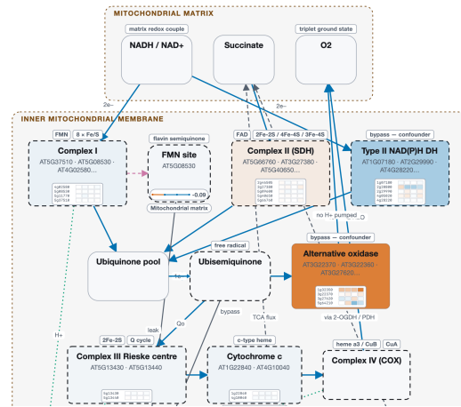
Figure 1: The atlas and its outputs. (A) QBM-01, the mitochondrial electron transport map, with evidence tier as a border channel: heavy solid T1, light solid T2, dashed T3, hairline T4. Most of the map is dashed. (B) Distribution of the 126 nodes across tiers — 72 % are T3 or T4, which is the state of the literature rather than a limitation of the corpus. (C) A near-null-field time course [18] projected onto the redox map; single-locus nodes carry a sparkline of the trajectory. (D) The same machinery under ionising radiation, where multi-locus nodes carry a per-locus heatmap instead — one row per locus, one column per timepoint. This is what reveals a gene family splitting, which the aggregate hides. Every panel is a file the repository generated; none was drawn. The browser tool is described in Section 2.6 rather than shown, because illustrating it would mean a screenshot rather than an artefact.
