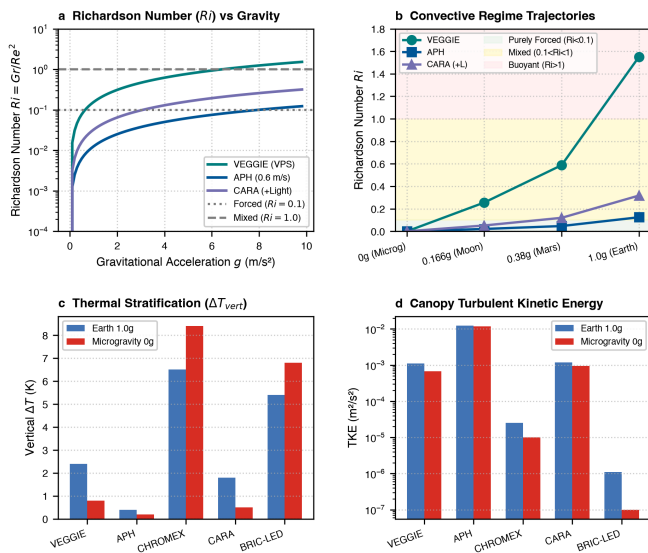
Figure 2 | Richardson number ( Ri ) scaling across gravity fields. a , Ri = \frac{Gr}{Re^2} trajectories from 1 g to 0 g. b , Convective regime trajectories. c , Thermal stratification. d , Turbulent kinetic energy (TKE).
