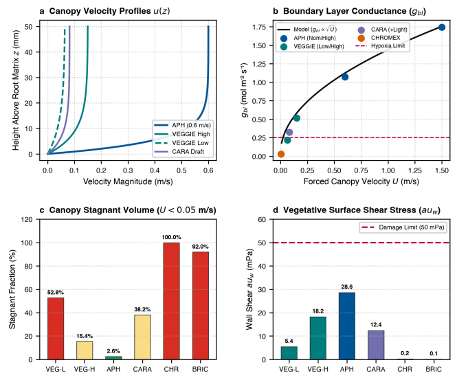
Figure 3 | Canopy boundary-layer conductance and turbulence. a , Vertical velocity profiles u(z) . b , g_{bl} vs forced velocity. c , Canopy stagnant volume fraction ( U < 0.05 m/s). d , Wall shear stress ( \tau_w ).
