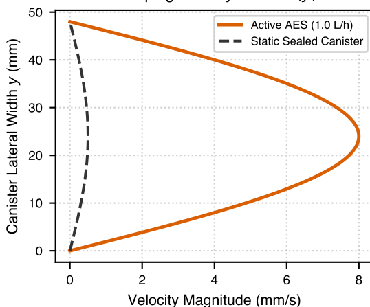
b PGC Creeping Velocity Profile u(y)
