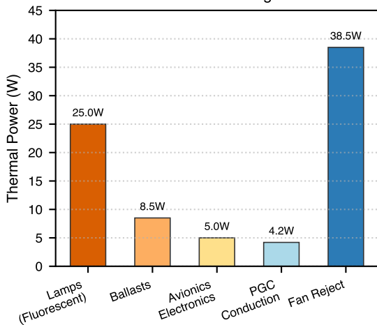
a PGU Chassis Thermal Budget
