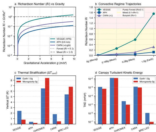
Figure 2 | Richardson number ( Ri ) scaling across gravity fields. a, Ri = \frac{Gr}{Re^2} trajectories from 1 g to 0 g. b, Convective regime trajectories. c, Thermal stratification. d, Turbulent kinetic energy (TKE).
