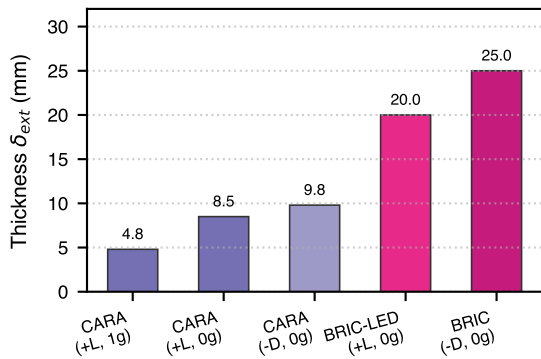
a External Boundary Layer \delta_{ext} (mm)
