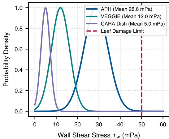
c Canopy Wall Shear Stress PDF
