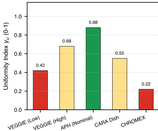
d Spatial Velocity Uniformity ( \gamma_u )
