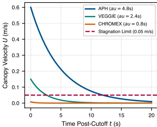
a Fan Spin-Down Velocity Decay U(t)
