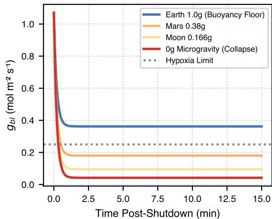
b Conductance Collapse across Gravities
