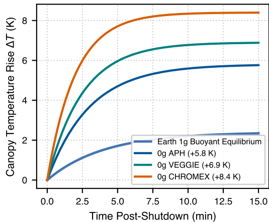
c Canopy Thermal Accumulation ( \Delta T )
