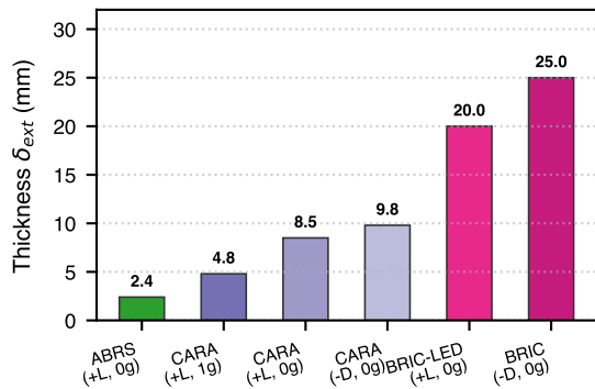
a External Boundary Layer \delta_{ext} (mm)
