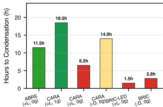
e Hours to 98% RH Condensation
