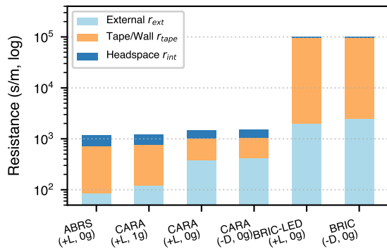
b Series Resistance r_{tot} = r_{ext} + r_{tape} + r_{int}
