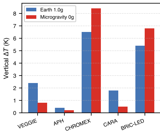
c Thermal Stratification ( \Delta T_{vert} )
