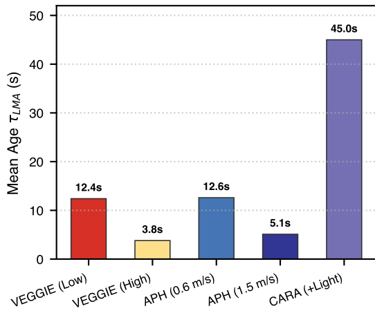
a Canopy Mean Age of Air (LMA)
