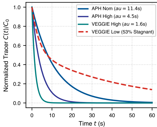
b Transient Scalar Flushing Kinetics
