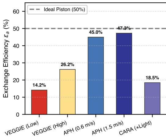
c Air Exchange Efficiency ( \varepsilon_a )
