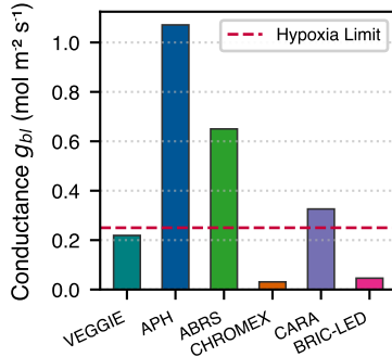
h \text{O}_2 Conductance g_{bl}
