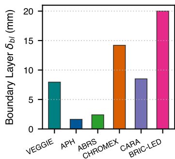
g \text{O}_2 Boundary Layer \delta_{bl} (mm)
