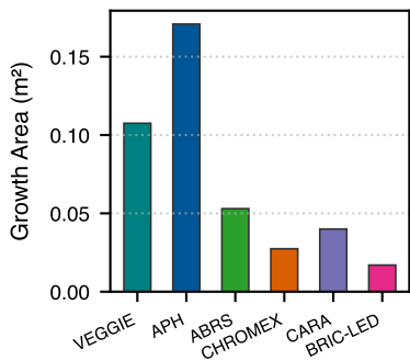
d Usable Growth Area ( \text{m}^2 )
