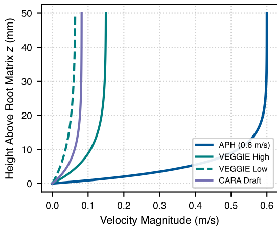
a Canopy Velocity Profiles u(z)
