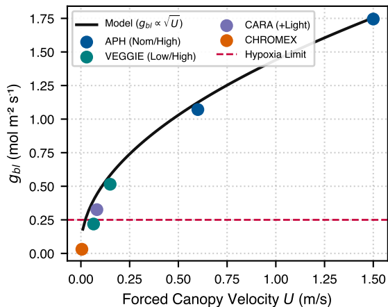
b Boundary Layer Conductance ( g_{bl} )
