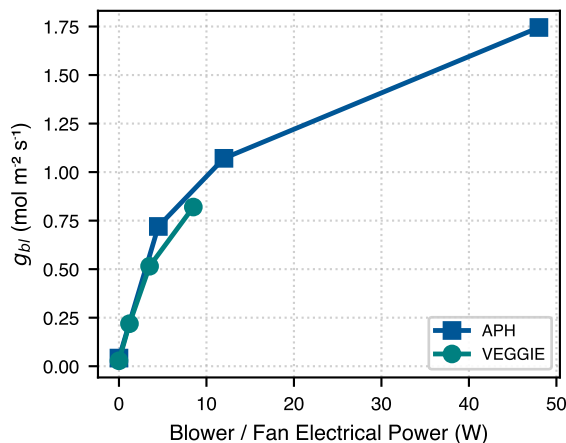
d Electrical Power vs g_{bl}
