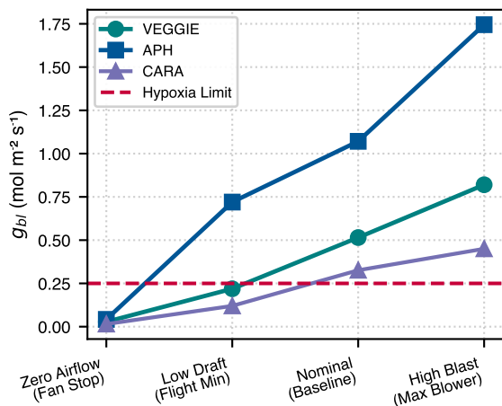
c Conductance g_{bl} Dynamic Range
