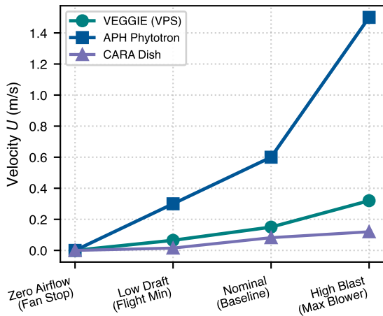
a Operational Canopy Velocities (m/s)
