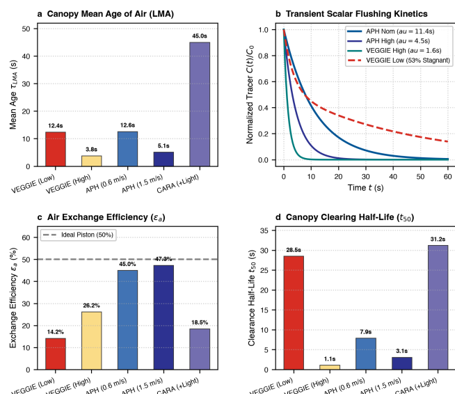
Figure 4 | Scalar ventilation dynamics, Local Mean Age of Air (LMA), and canopy dead zone mapping. a, Mean Age of Air (LMA). b, Transient scalar flushing decay \frac{C(t)}{C_0} . c, Air exchange efficiency ( \epsilon_a ). d, Clearing half-life ( t_{50} ).
