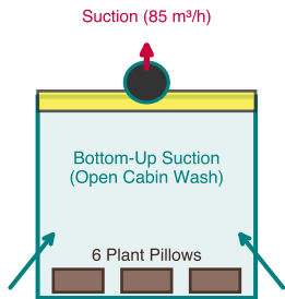
a VEGGIE / VPS (37.6 L)
