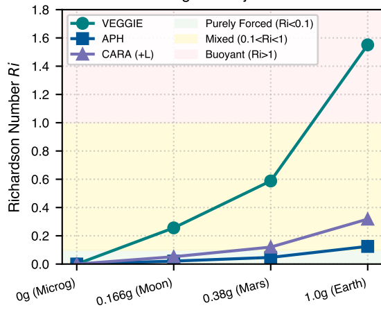
b Convective Regime Trajectories
