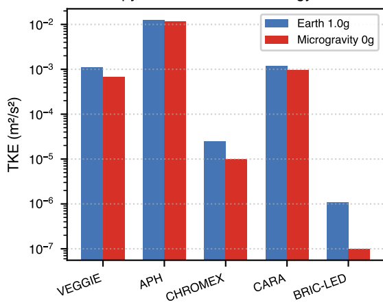
d Canopy Turbulent Kinetic Energy
