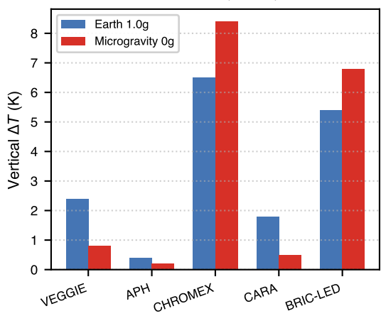
c Thermal Stratification ( \Delta T_{vert} )
