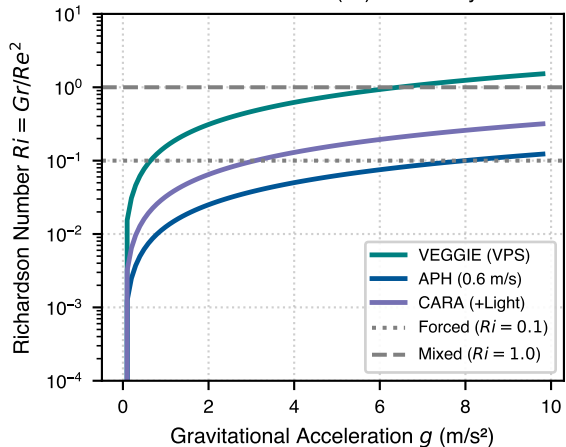
a Richardson Number ( Ri ) vs Gravity
