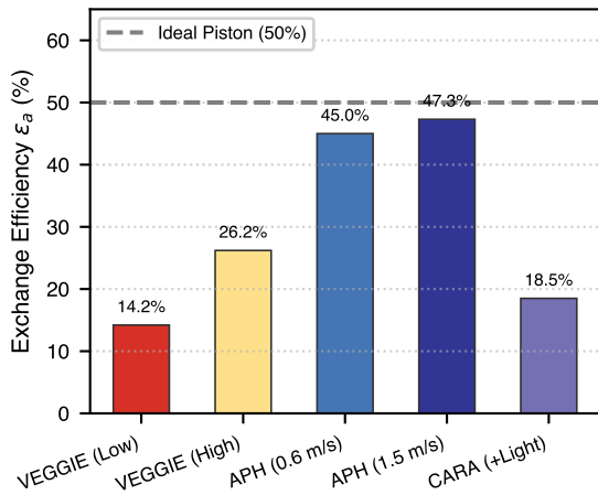
c Air Exchange Efficiency ( \epsilon_a )
