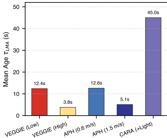
a Canopy Mean Age of Air ( \tau_{LMA} )
