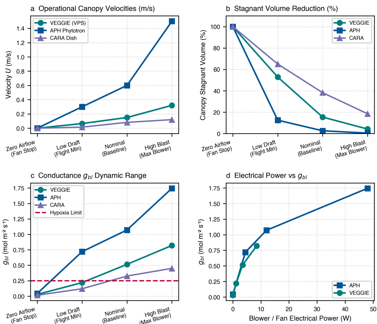
Figure 7 | Operational airflow extremes and stagnation regimes across spaceflight plant growth hardware in microgravity. a, Operational canopy velocities. b, Stagnant volume reduction vs fan speed. c, Conductance ( g_{bl} ) across operating modes. d, Aerodynamic conductance vs fan electrical power.
