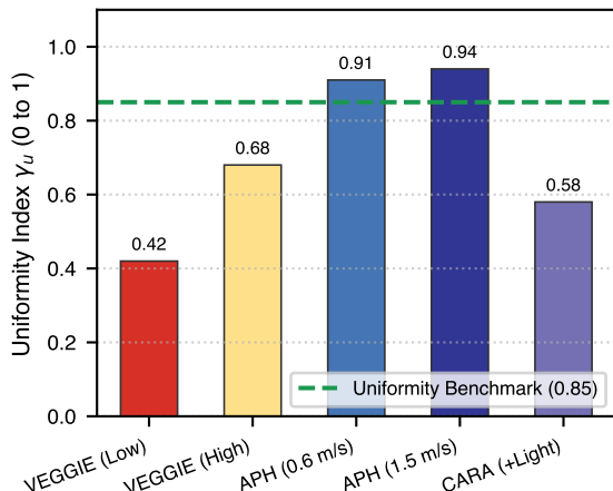
d Spatial Velocity Uniformity Index ( \gamma_u )
