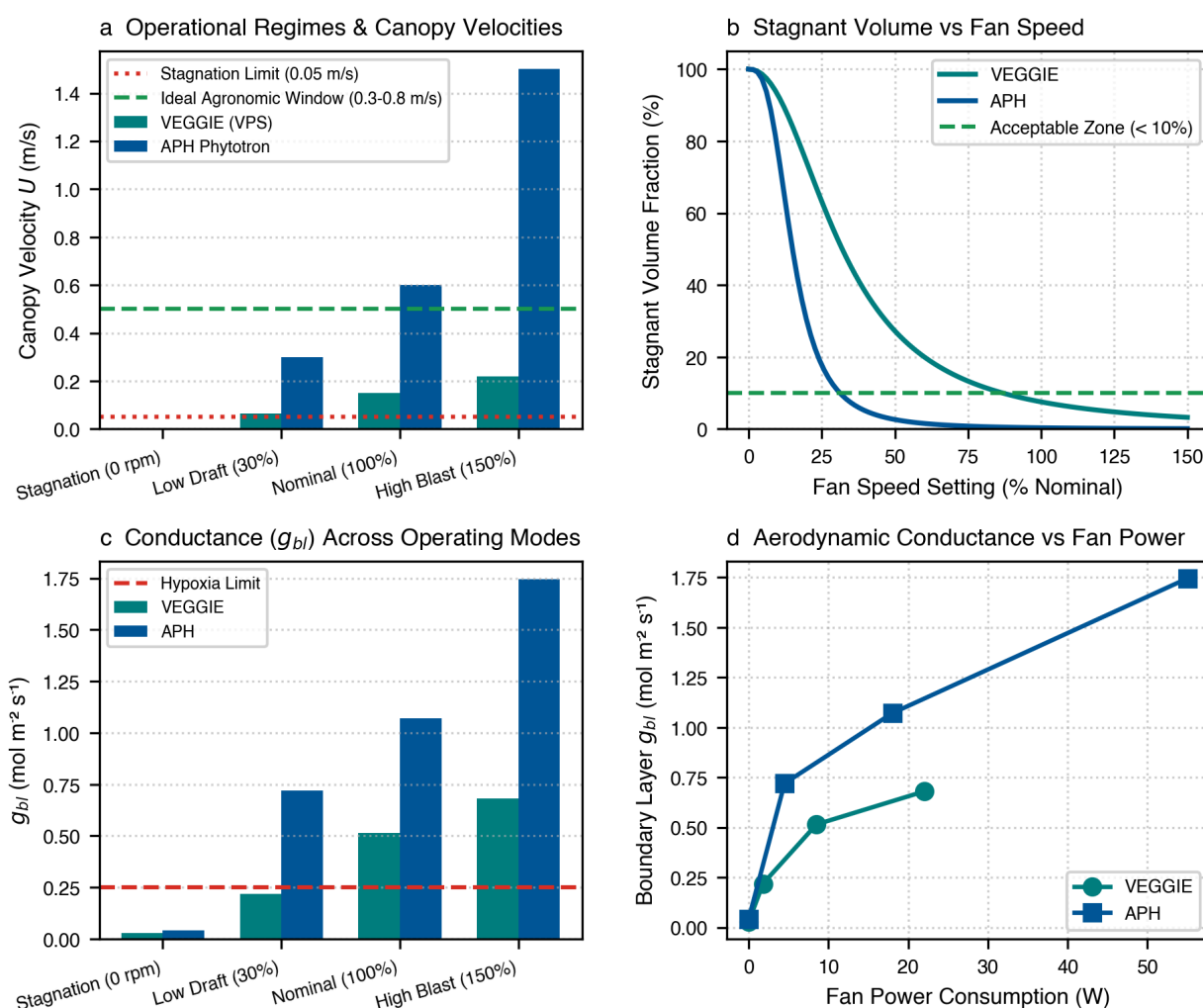
Figure 7 | Operational airflow extremes and stagnation regimes across spaceflight plant growth hardware in microgravity. a , Operational canopy velocities. b , Stagnant volume reduction vs fan speed. c , Conductance ( g_{bl} ) across operating modes. d , Aerodynamic conductance vs fan electrical power.
