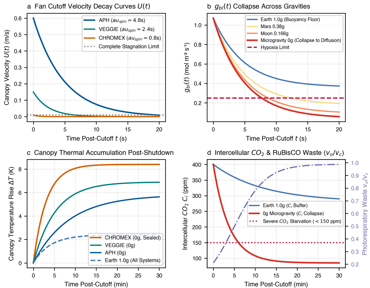
Figure 9 | Transient aerodynamics of fan failure, boundary-layer collapse, and physiological starvation across gravitational fields. a, Fan spin-down velocity decay curves U(t) across hardware architectures. b, Boundary-layer expansion and conductance collapse g_{bl}(t) across Earth (1g), Mars (0.38g), Moon (0.166g), and Microgravity (0g). c, Canopy thermal accumulation post-shutdown. d, Intercellular CO_2 drawdown ( C_i ) and photorespiratory oxygenation surge ( v_o/v_c ).
