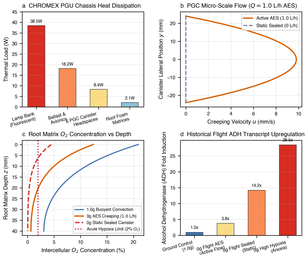
Figure 8 | NASA Space Shuttle CHROMEX / PGU multi-scale thermal-fluid dynamics, PGC creeping flow, and hypoxia transcriptomic linkage. a , Macro PGU Middeck locker chassis heat dissipation (38.5 W fluorescent lamps). b , Micro PGC canister creeping velocity profile u(y) under active AES (1.0 L/h) vs static sealed conditions. c , Root matrix O_2 concentration profiles vs depth ( z , mm) under Brinkman-Darcy porous flow. d , Correlation to historical CHROMEX-03 flight transcriptomics: upregulation of alcohol dehydrogenase (ADH) under unstirred boundary layer hypoxia ( O_2 < 5\% ).
