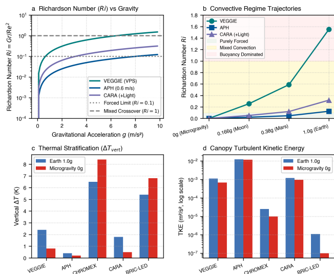
Figure 2 | Richardson number ( Ri ) scaling across gravity fields. a, Ri = \frac{Gr}{Re^2} trajectories from 1 g to 0 g. b, Convective regime trajectories. c, Thermal stratification. d, Turbulent kinetic energy (TKE).
