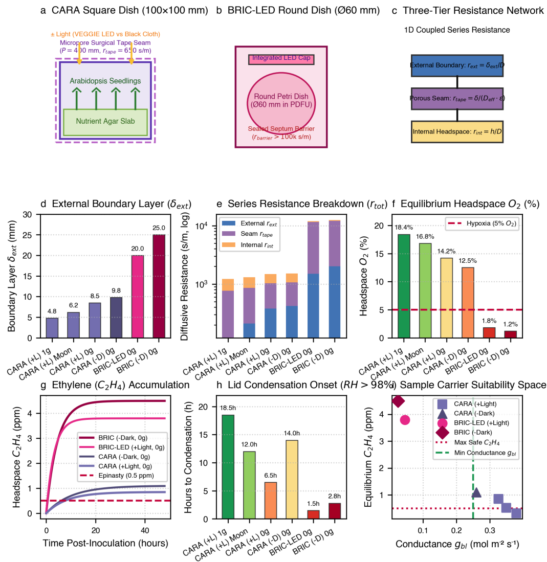
Figure 10 | Petri dish science sample carrier microenvironments: CARA square dishes ( \pm Light) vs BRIC / BRIC-LED round dishes ( \pm Light) across spaceflight hardware. a , CARA square dish (100 × 100 × 20 mm, P = 400 mm) with micropore surgical tape perimeter seam. b , BRIC-LED round dish (Ø60 × 15 mm) in sealed PDFU canister with integrated LED cap. c , Three-tier series resistance network ( r_{ext} + r_{tape/barrier} + r_{int} ). d , External boundary layer thickness ( \delta_{ext} ). e , Series resistance breakdown ( r_{tot} ). f , Headspace oxygen concentration ( O_2 ). g , Ethylene accumulation ( C_2H_4 ). h , Hours to 98% RH droplet condensation. i , Sample carrier suitability space.
