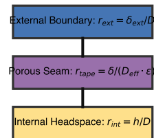
1D Coupled Series Resistance
