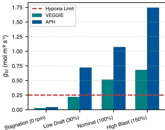
c Conductance ( g_{bl} ) Across Operating Modes
