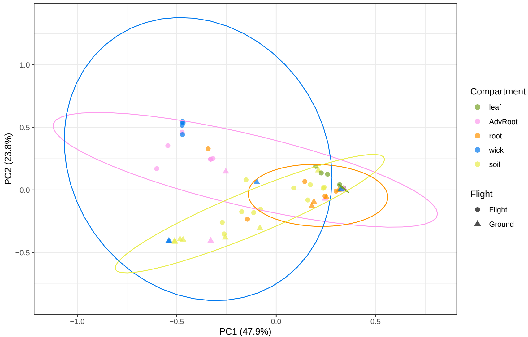
Bray-Curtis PCoA (ITS)
