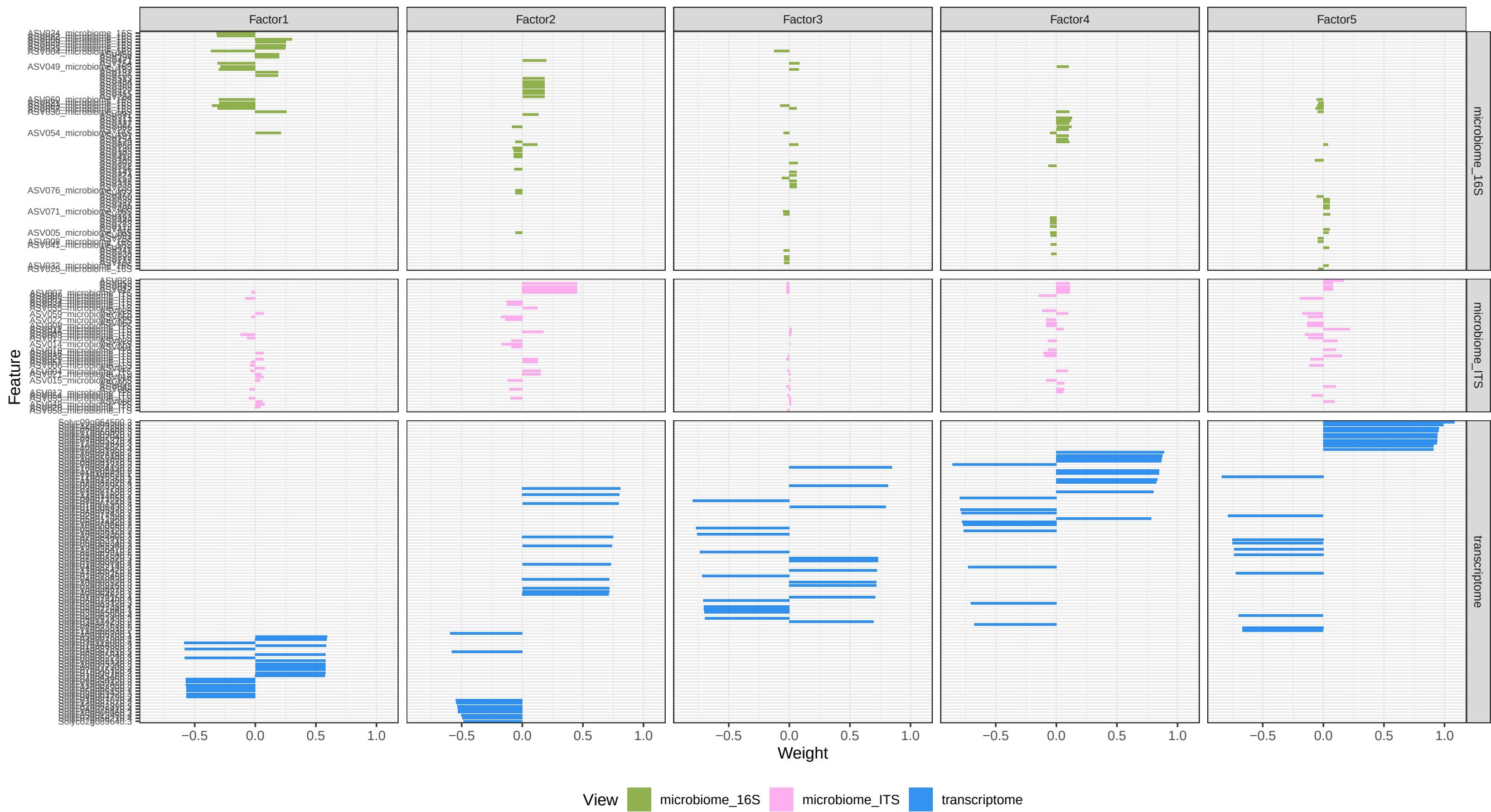
MOFA+ Top Feature Weights per Factor
