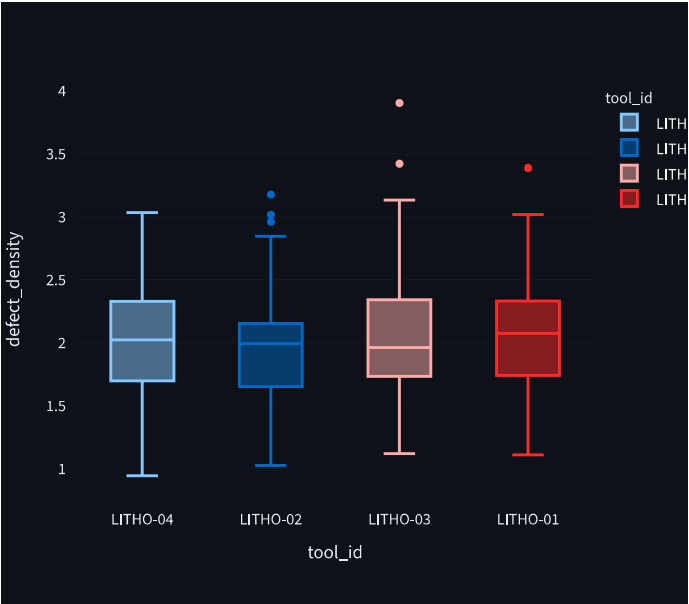
Defect Density by Tool
