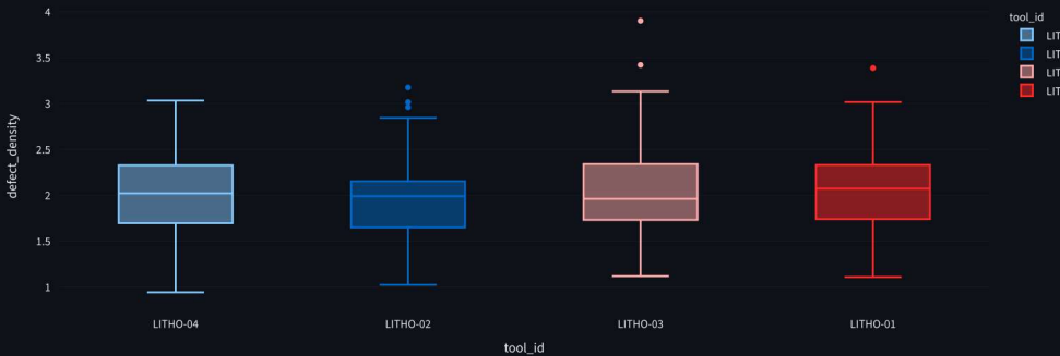
Defect Density by Tool
