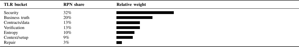
Fig. 2. TLR means Top-Level Risk. Shares are computed directly from Table VI: each row contributes its RPN to one TLR bucket, then bucket totals are rounded to whole percentages. The chart is a policy-priority model for Jankurai 0.7.0, not an incident-frequency measurement.
